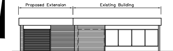
SIDE ELEVATION
